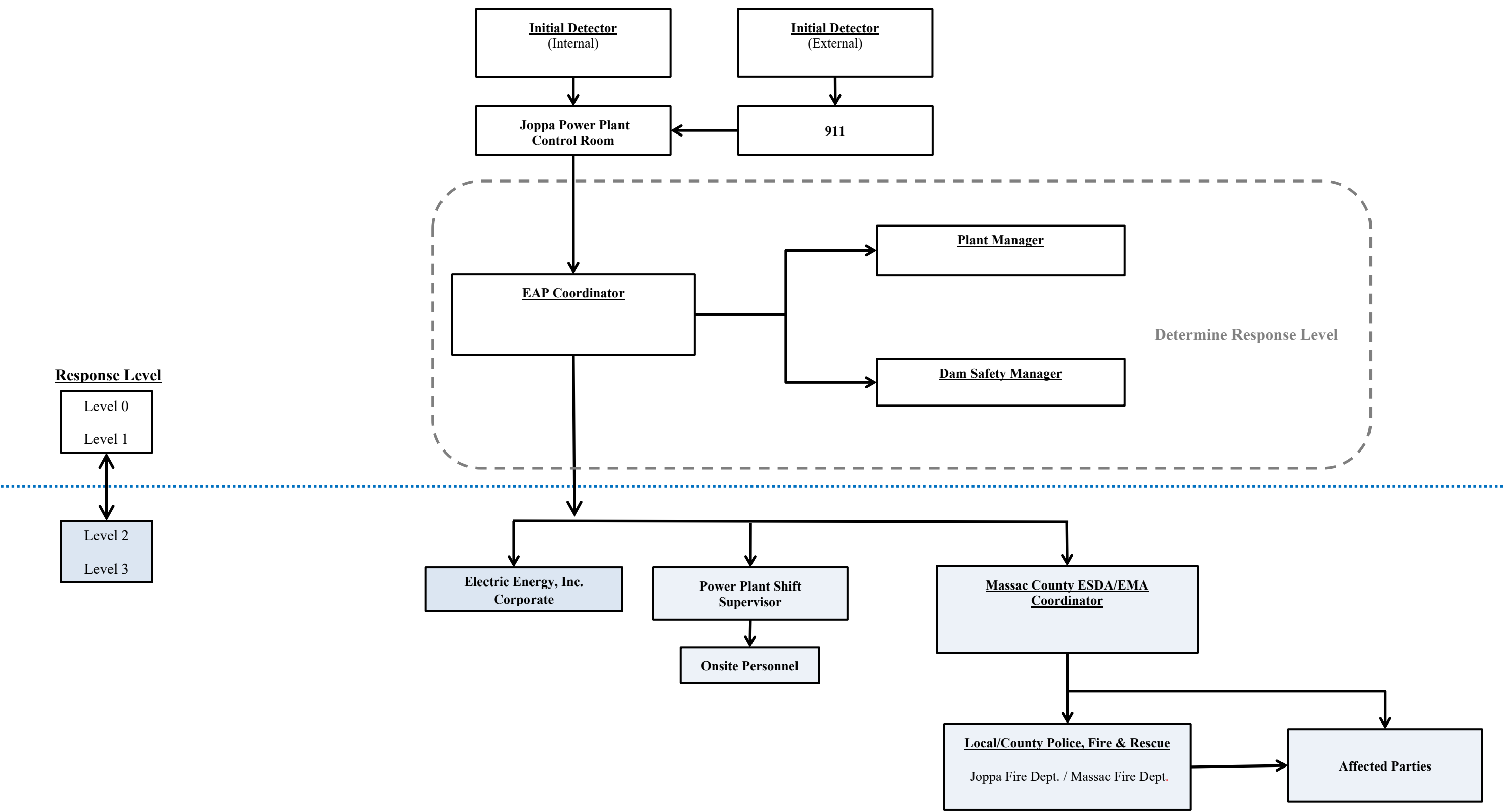
Figure 2-2. Notification Flowchart
